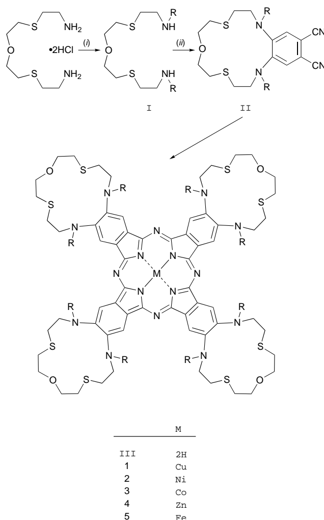
Scheme 1 R = p -MeC 6 H 4 SO 2 . (i) p -MeC 6 H 4 SO 2 Cl, CH 2 Cl 2 , NaOH, water; (ii) 1,2-dichloro-4,5-dicyanobenzene, dmf, K 2 CO 3 , 50 °C
